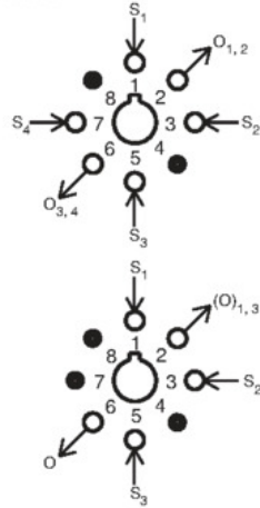
R-603 3-Input "OR"
