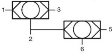
R-603 3-Input "OR"
