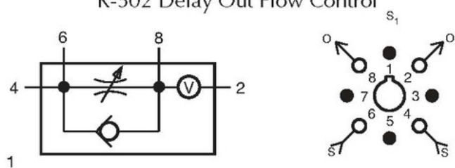
R-502 Delay Out Flow Control
