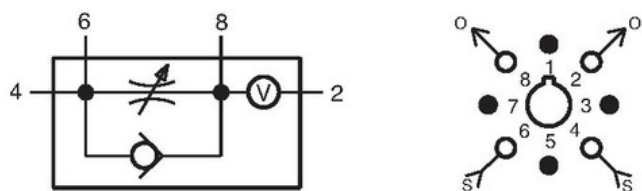
R-502 Delay Out Flow Control
