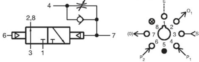
Delayed In Normally-Open
