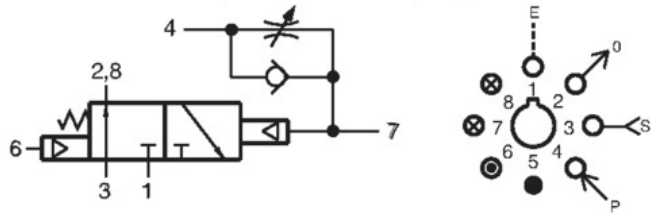
Delayed In Normally-Open
