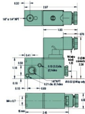
2-Way & 3-Way Valves (stacking)
