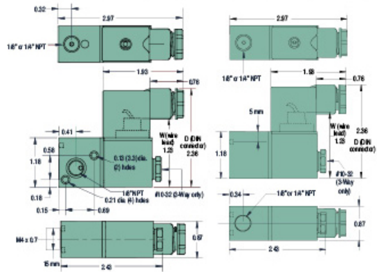
2-Way & 3-Way Valves (stacking) 2-Way & 3-Way Valves (non-stacking)
