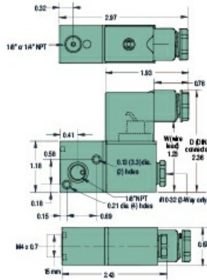
2-Way & 3-Way Valves (stacking)
