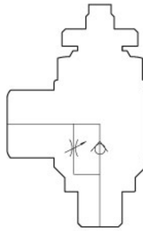
meter out (A)
