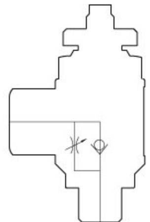
meter in (B)
