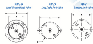
DIMENSIONS, NPV-P (Panel Mounted Pinch Valves)
