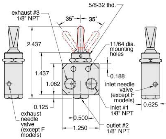
Fill & Bleed Valve, Momentary/Momentary, Full Adj., #10-32
