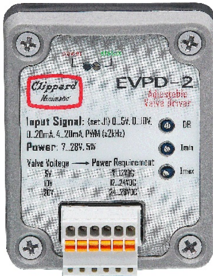
EV-P Series Proportional Valve Driver, Board with Housing
