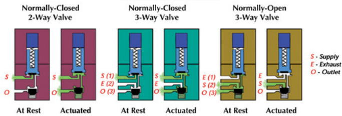
FUNCTIONAL SCHEMATICS
