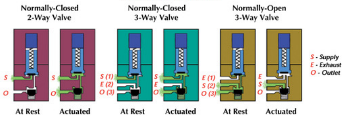
FUNCTIONAL SCHEMATICS
