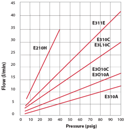
Typical Air Flow
