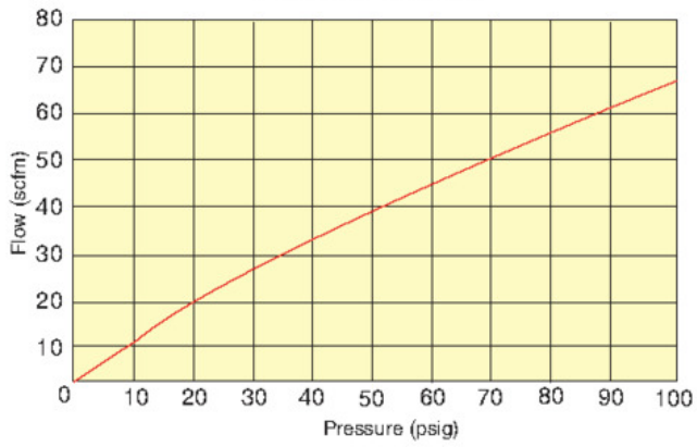
Pressure vs. Flow
