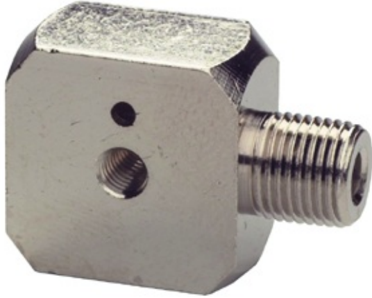
2-Station Manifold, 1/8" NPT Inlet / #10-32 Outlet
